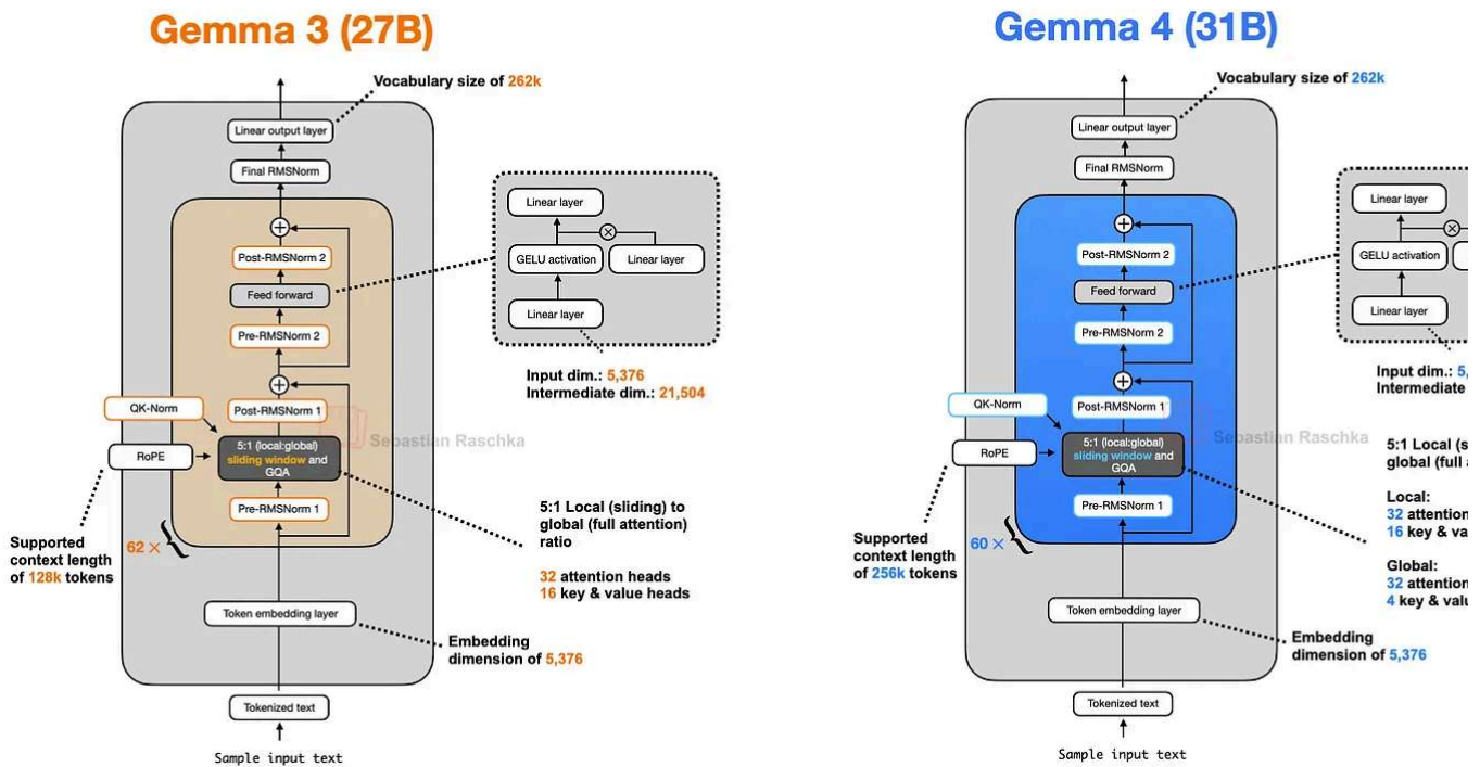
Figure 58: Gemma 3 (27B) and Gemma 4 (31B) side by side.
