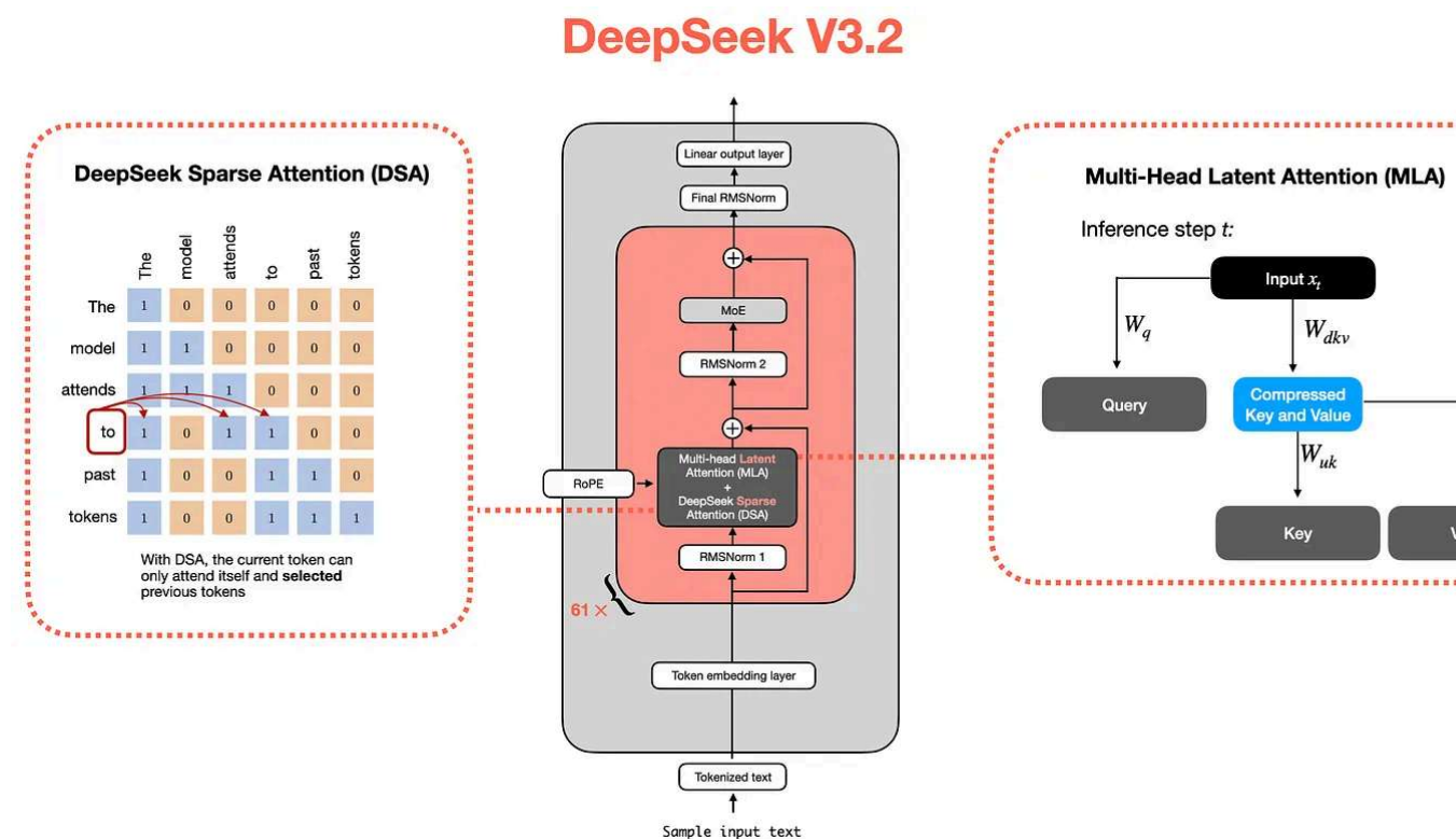
Figure 48: The DeepSeek model architecture with multi-head latent and sparse attention.
