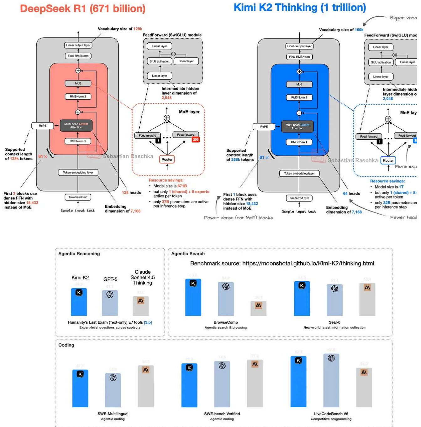
Figure 25.2: DeepSeek R1 versus Kimi K2 Thinking architecture (top) and Kimi K2 Thinking benchmarks (bottom).
