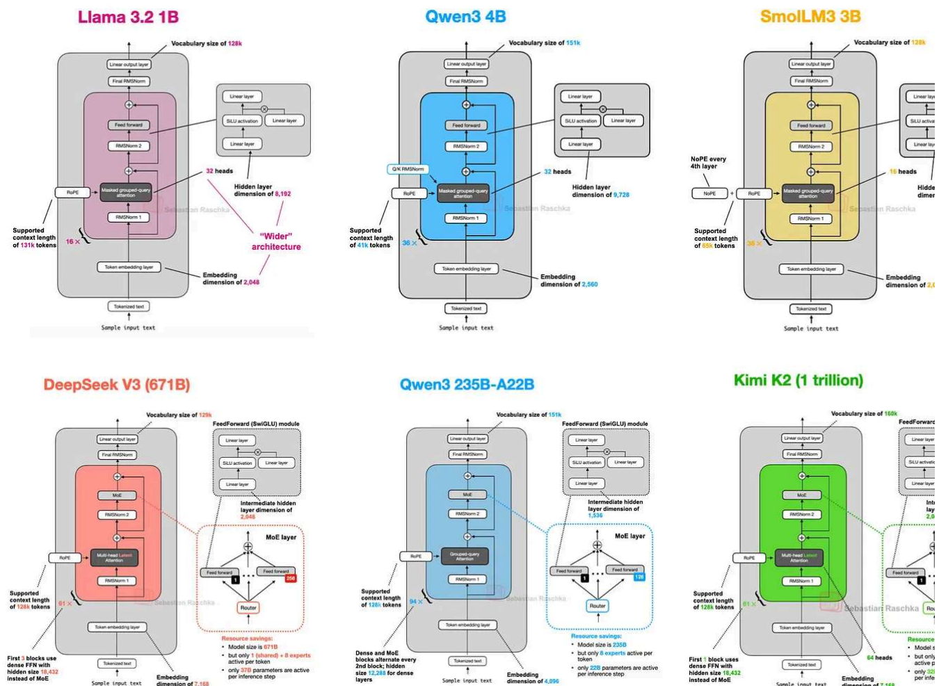
Figure 1: A subset of the architectures covered in this article.
