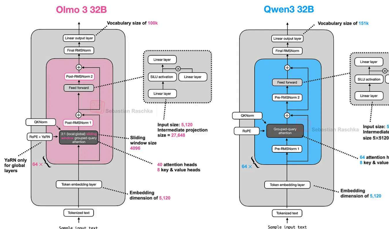
Figure 45: Olmo 3 32B and Qwen3 32B side by side.
