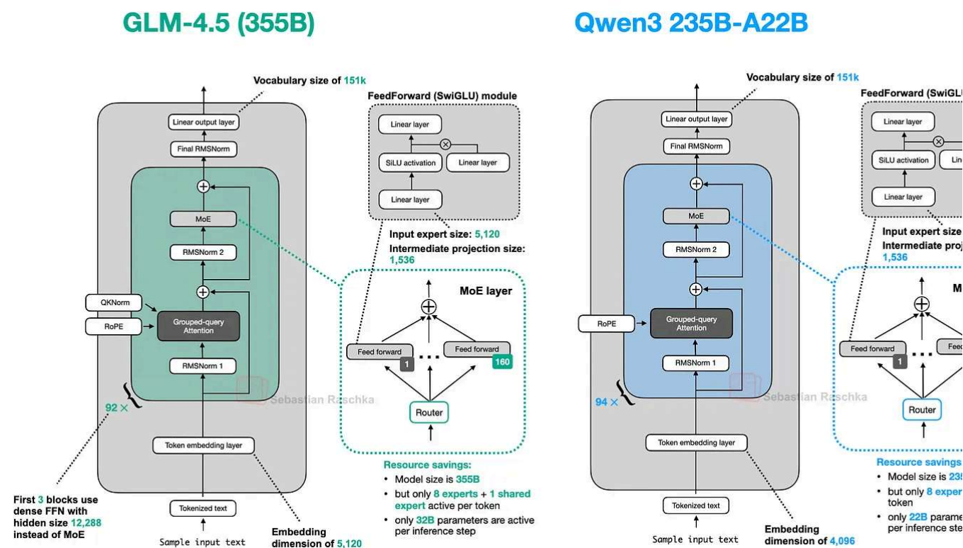
Figure 34: GLM-4.5 next to a similarly-sized Qwen3 model.
