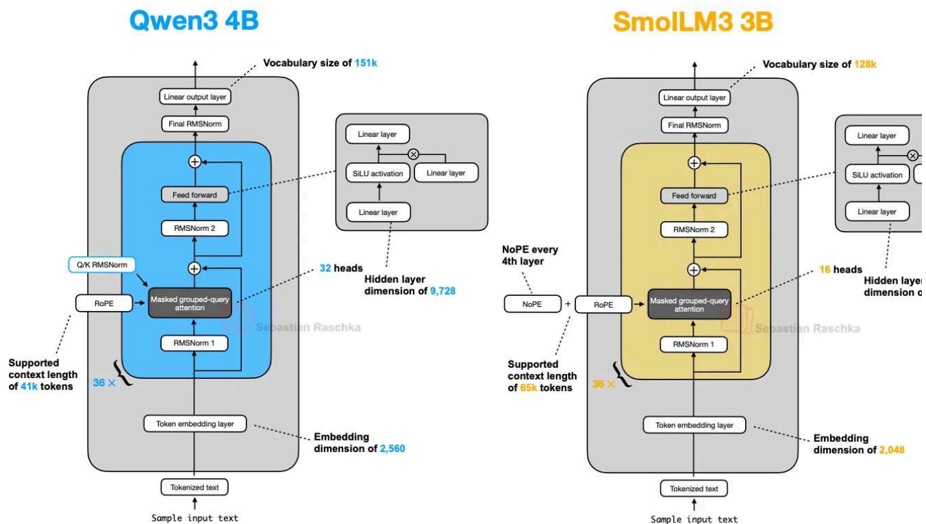
Figure 21: A side-by-side architecture comparison between Qwen3 4B and SmolLM3 3B.
