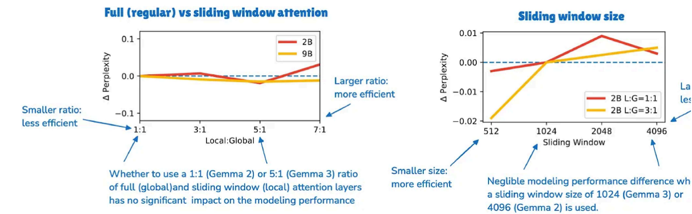
Figure 13: An annotated figure from Gemma 3 paper ( https://arxiv.org/abs/2503.19786 ) showing that sliding window attention has little to no impact on the LLM-generated output perplexity.
