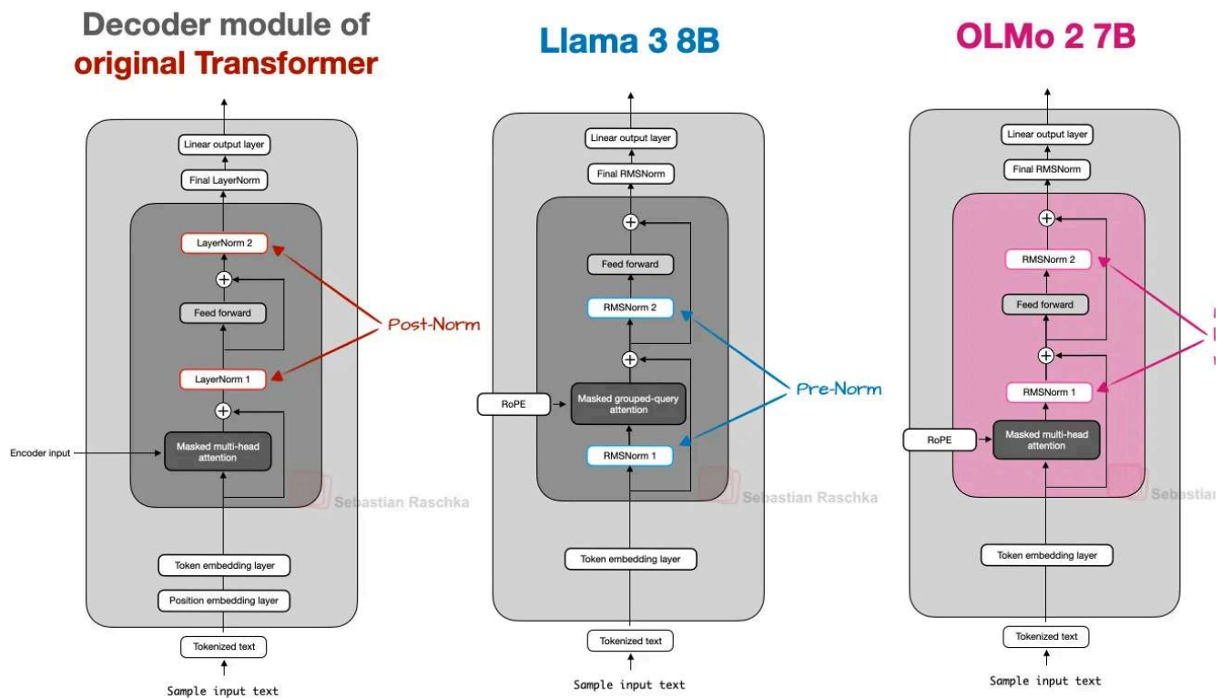
Figure 8: A comparison of Post-Norm, Pre-Norm, and OLMo 2's flavor of Post-Norm.
