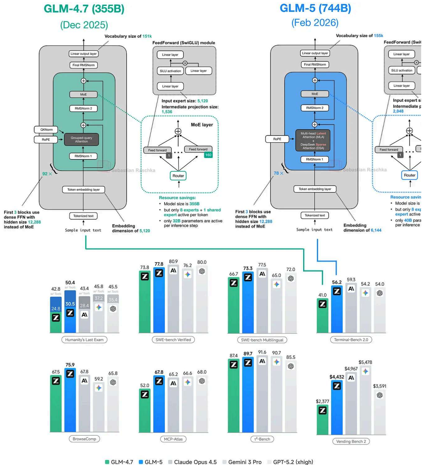
Figure 57: GLM architectures next to benchmarks. The GLM-4.7 architecture is similar to GLM-4.5. The benchmarks are taken from the GLM-5 release blog post: https://z.ai/blog/glm-5
