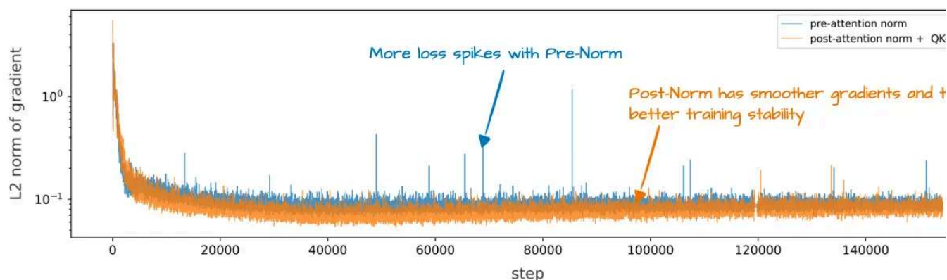
Figure 9: A plot showing the training stability for Pre-Norm (like in GPT-2, Llama 3, and many others) versus OLMo 2's flavor of Post-Norm. This is an annotated figure from the OLMo 2 paper, https://arxiv.org/abs/2501.00656
