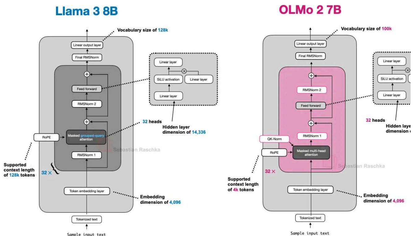
Figure 10: An architecture comparison between Llama 3 and OLMo 2.
